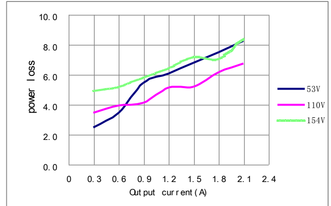
Figure 2: Power dissipation vs. load current for 53, 110 and 154 input voltage at 25°C.
