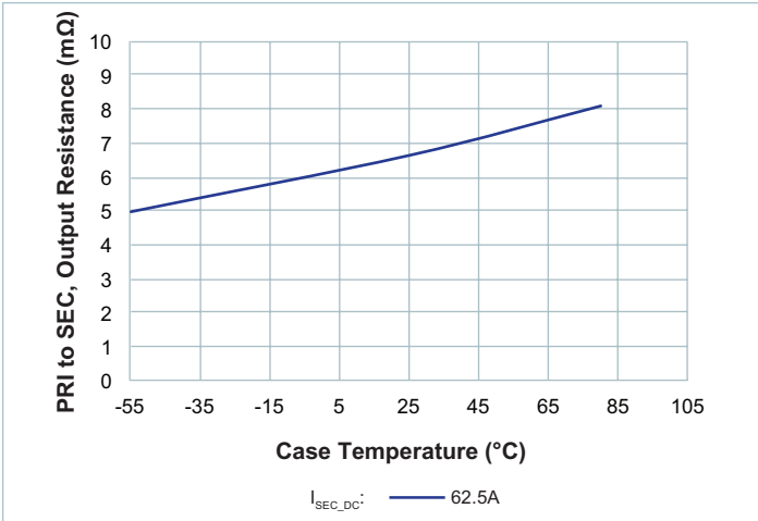
Figure 12 — R_SEC vs. temperature; nominal V_PRI_DC I_SEC_DC = 62.5A at T_CASE = 80°C
