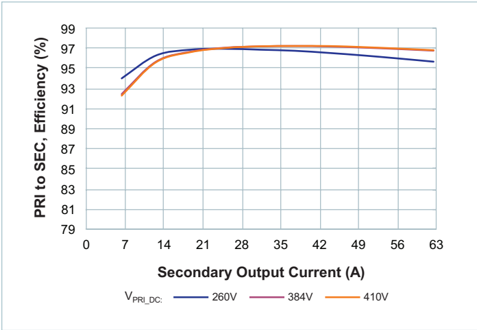
Figure 10 — Efficiency at T_CASE = 80°C
