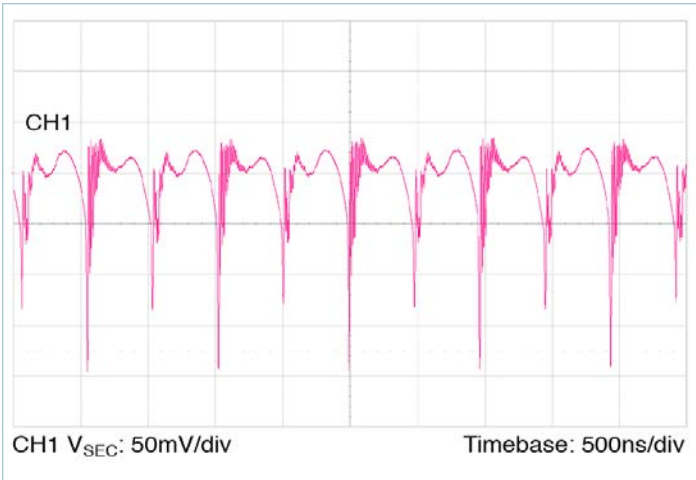
Figure 14 — Full-load secondary voltage ripple, 10µF C_PRI_IN_EXT; no external C_SEC_OUT_EXT. Board-mounted module, scope setting: 20MHz analog BW
