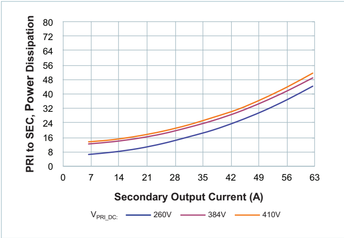
Figure 11 — Power dissipation at T_CASE = 80°C
