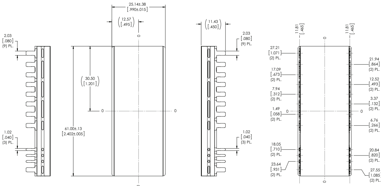
TOP VIEW (COMPONENT SIDE) BOTTOM VIEW
