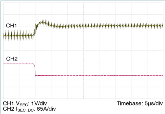
Figure 16 — 62.5 – 0A transient response: C_{PRI\_IN\_EXT} = 10\mu F , no external C_{SEC\_OUT\_EXT}
