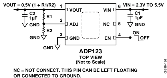
Figure 4. ADP123 with Adjustable Output Voltage (LFCSP Version)
