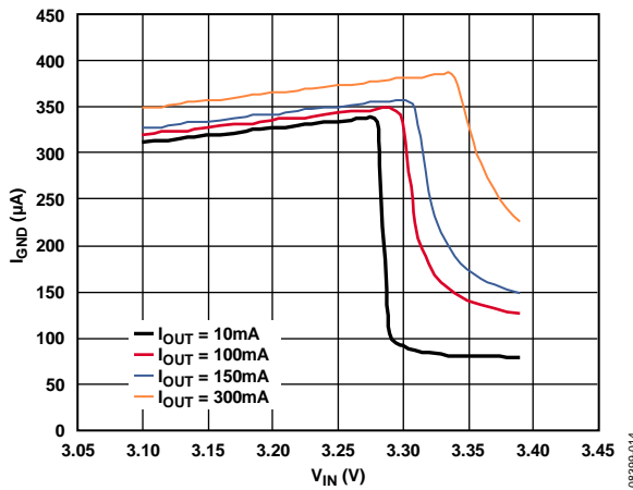
Figure 17. Ground Current vs. Input Voltage (in Dropout)
