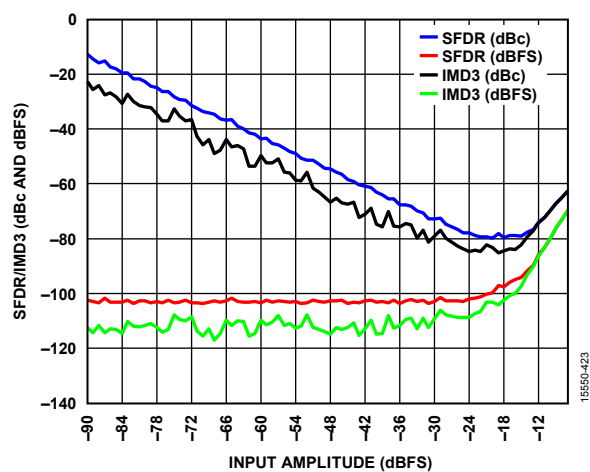
Figure 23. Two-Tone SFDR/IMD3 vs. Input Amplitude ( A_{IN} ) with f_{IN1} = 2137.5 MHz, f_{IN2} = 2142.5 MHz
