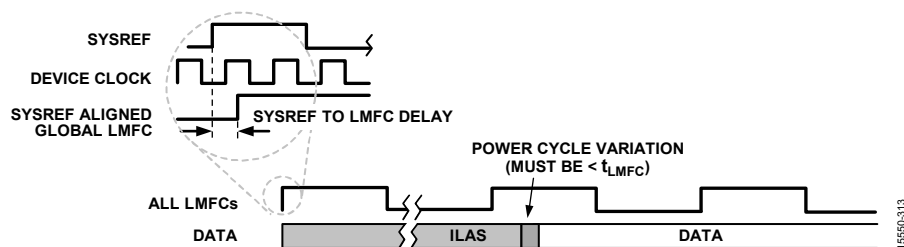
Figure 143. SYSREF and LMFC
