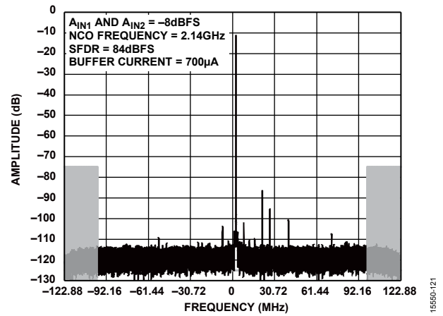
Figure 51. Two-Tone FFT; f_{IN1} = 1846.5\text{ MHz} , f_{IN2} = 2142.5\text{ MHz} ; f_{CLK} = 2.4576\text{ GHz} ; Decimation Ratio = 10, NCO Frequency = 2140 MHz
