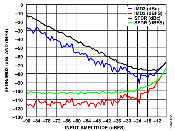
Figure 52. Two-Tone SFDR/IMD3 vs. Input Amplitude ( A_{IN} ) with f_{IN1} = 1841.5\text{ MHz} , f_{IN2} = 1846.5\text{ MHz}
