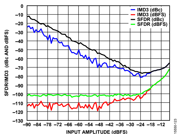
Figure 53. Two-Tone SFDR/IMD3 vs. Input Amplitude ( A_{IN} ) with f_{IN1} = 2137.5\text{ MHz} , f_{IN2} = 2142.5\text{ MHz}
