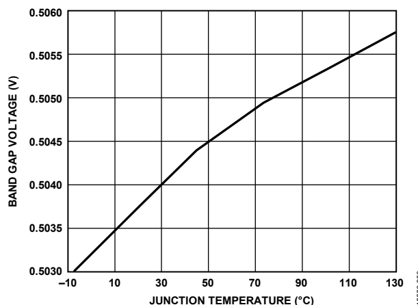
Figure 84. Typical Reference Voltage ( V_{REF} ) Drift
