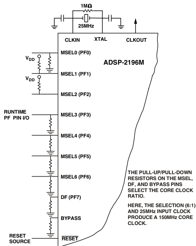
Figure 3. External Crystal Connections
