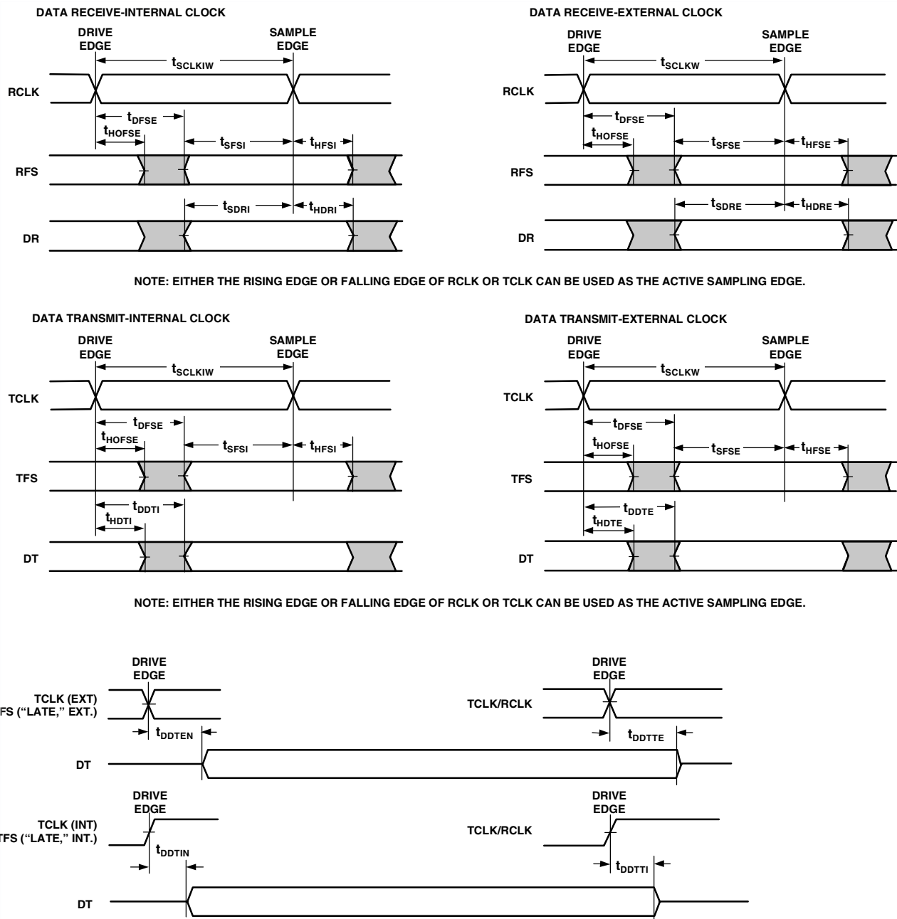
Figure 18. Serial Ports
