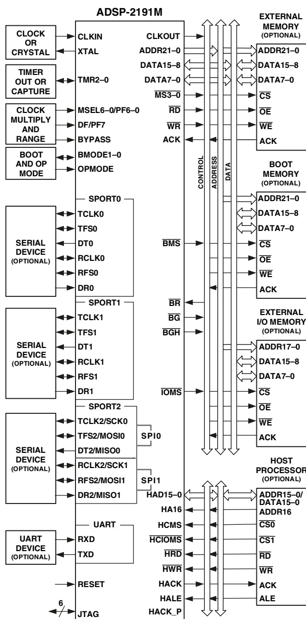
Figure 1. System Diagram
