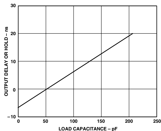
Figure 30. Typical Output Delay or Hold vs. Load Capacitance (at Maximum Case Temperature) To ensure that the T_{AMB} data sheet specification is not exceeded, a heatsink and/or an air flow source may be used. A heatsink should be attached to the ground plane (as close as possible to the thermal pathways) with a thermal adhesive.
