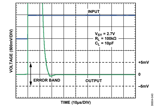
Figure 52. Positive Settling Time to 0.1%
