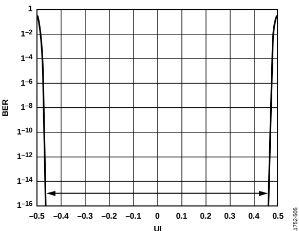
Figure 166. Digital Outputs Bathtub Curve, External 100 Ω Terminations at 6 Gbps
