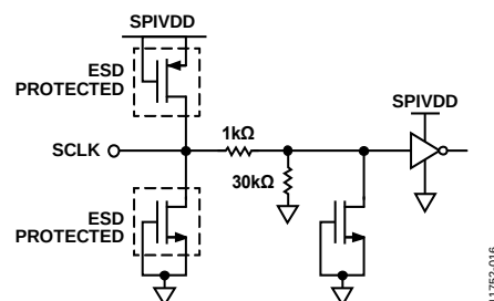
Figure 109. SCLK Input
