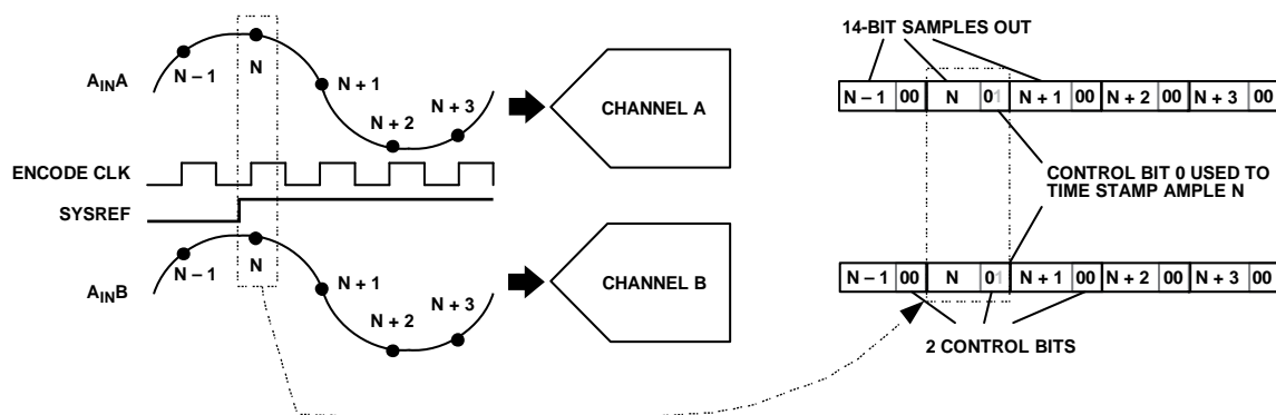
Figure 174. AD9680 Timestamping—CS = 2 (Register 0x58F, Bits[7:6] = 2), Control Bit 1 is SYSREF± (Register 0x559, Bits[6:4] = 5)
