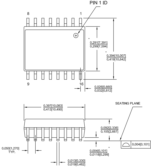
Figure 46. 16-pin SOIC (0.413 × 0.299 × 0.0932) Inches Package Outline, 51-85022
