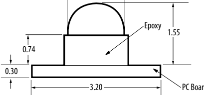
HSMx-C380
