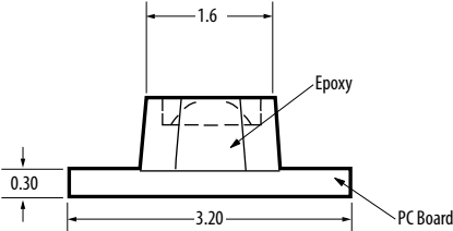
HSMx-C350
