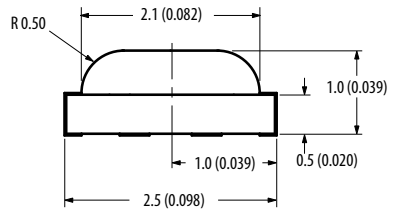
HSMF-C113/C115
