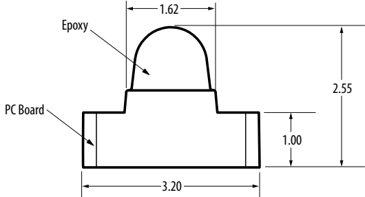
HSMx-C400
