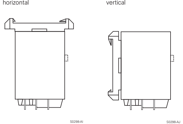
Cover with DIN-snap-on attachment (FASTON 250 only)
