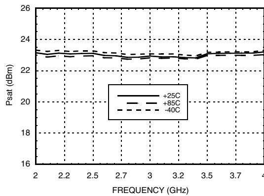
Psat vs. Temperature [1]
