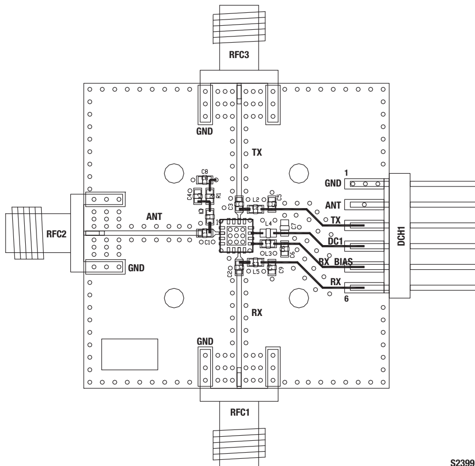
Figure 22. SKY12208-306LF Evaluation Board Assembly Diagram
