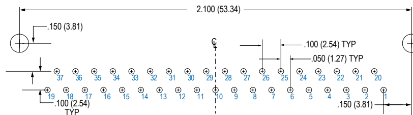
37 PIN MWDM-37PBR
