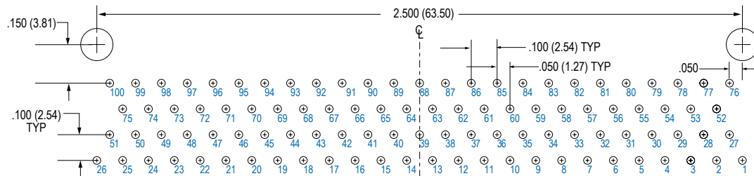
100 PIN MWDM-100PBR
