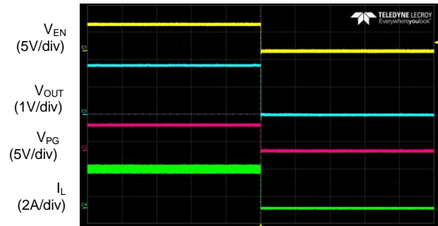
Enable Turn off Characteristic (I OUT =3A)
