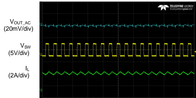
Output Ripple (I OUT =3A)
