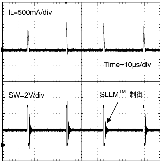
Figure 36. Switching Waveform with SLLM™ (VIN = 3.3V, VOUT = 1.8V, IOUT = 30mA, L=1.5µH)
