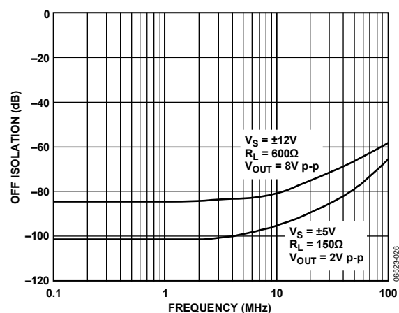
Figure 34. Off Isolation vs. Frequency
