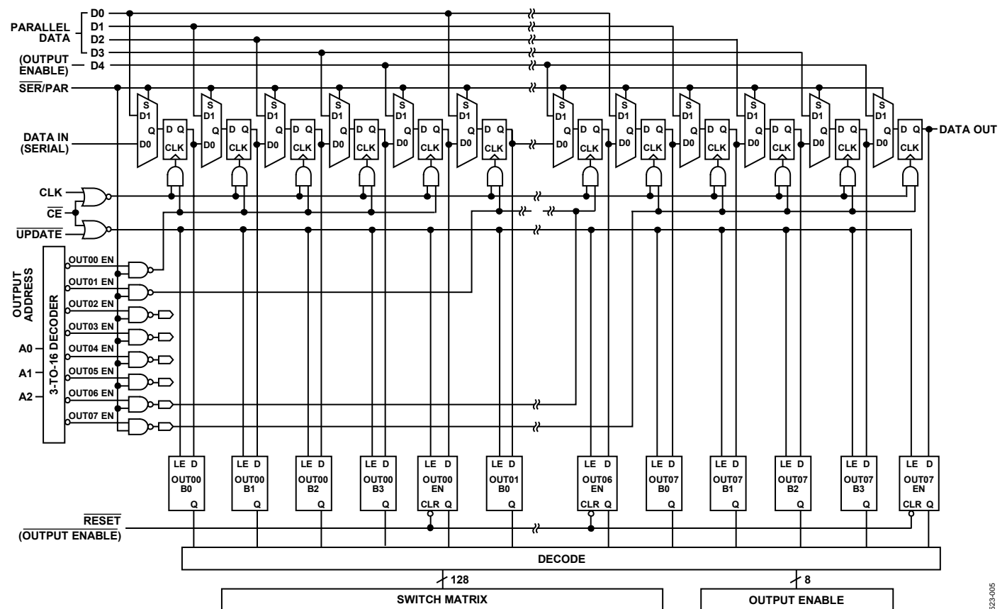
Figure 5. Logic Diagram
