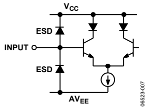
Figure 7. Analog Input
