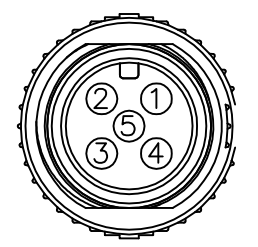
Conn.1 Pin Assignments Front View
