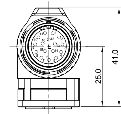
E type, Normal Key
