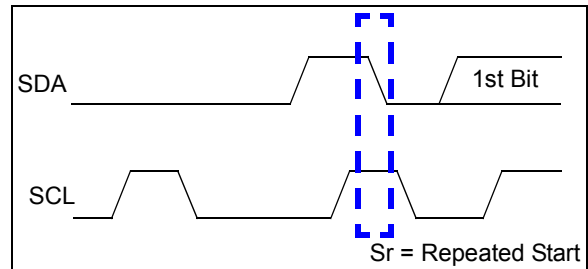
FIGURE 5-5: Repeat Start Condition Waveform.
