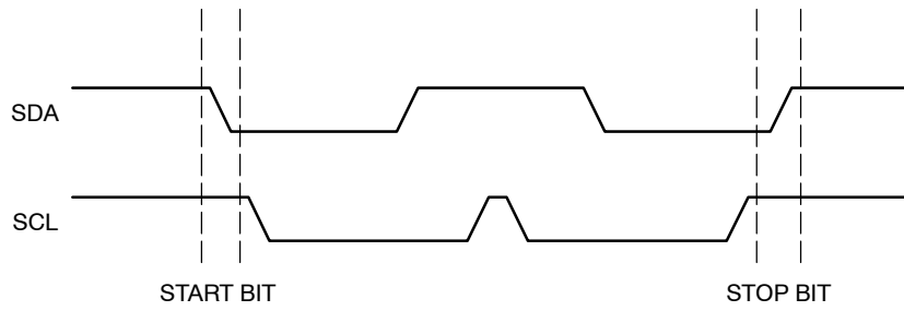
Figure 20. Start/Stop Timing
