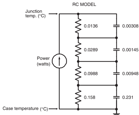
FIGURE 2, TRANSIENT THERMAL IMPEDANCE MODEL
