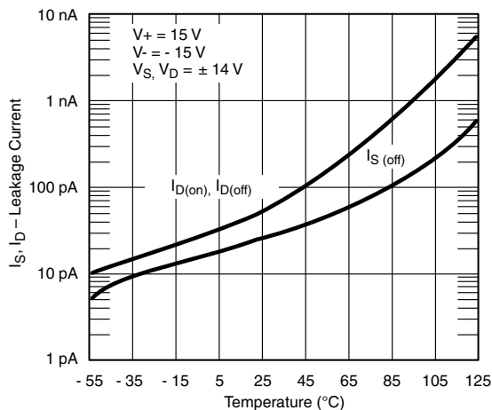
I D , I S Leverages vs. Temperature
