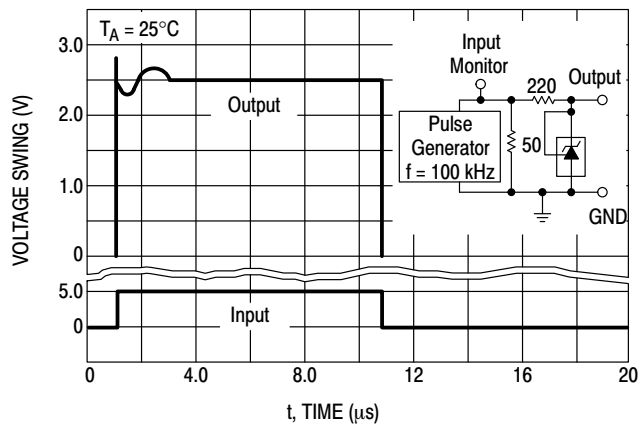
Figure 14. Pulse Response
