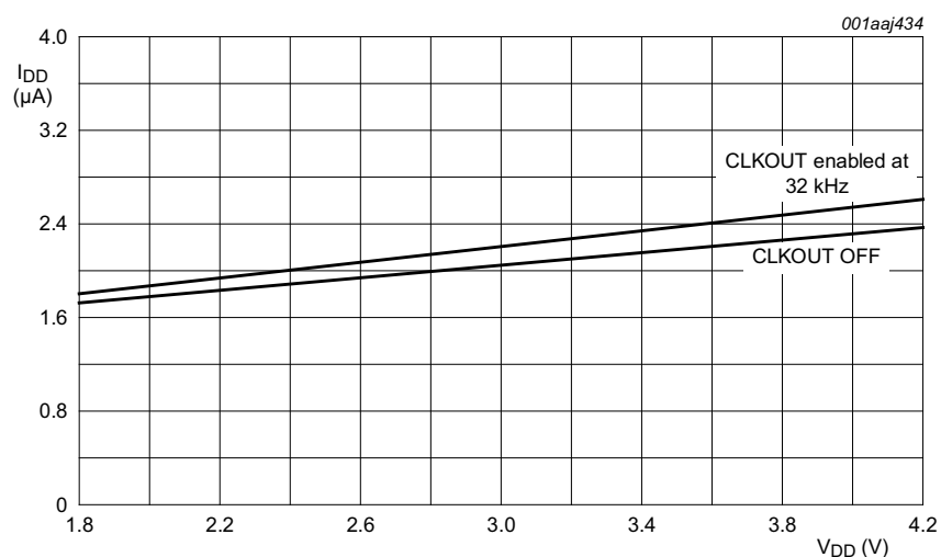
Fig 51. I_{DD} as a function of V_{DD}
