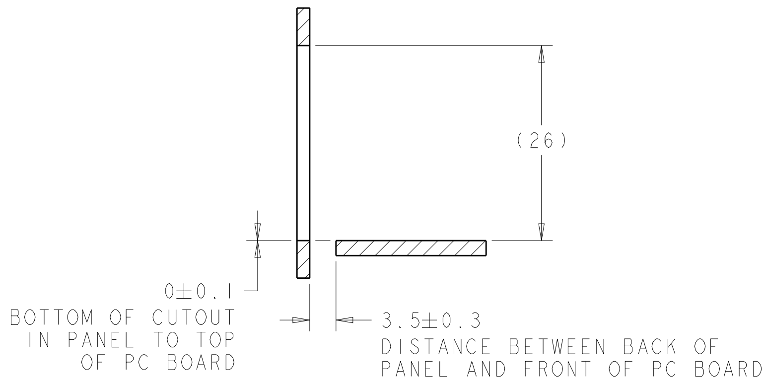
SECTION U-U
