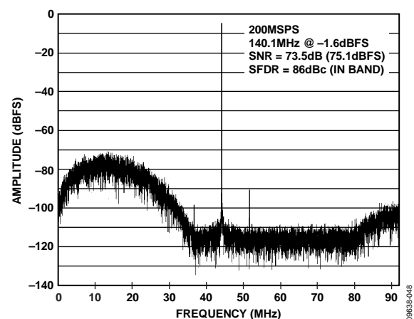
Figure 55. 22% BW Mode, Tuning Word = 41
