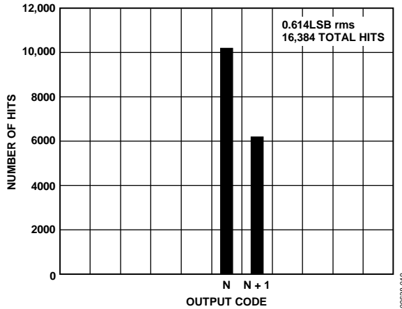
Figure 19. AD6643-200 Grounded Input Histogram
