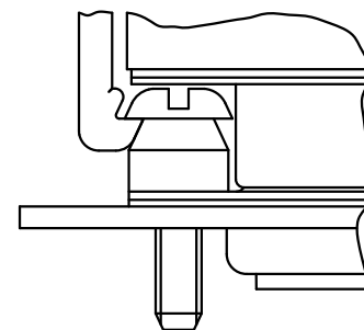
Front mounted connector example
