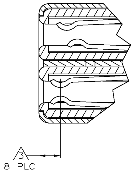
DETAIL D SCALE 10:1
