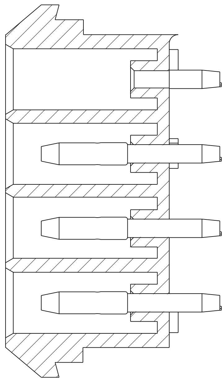
SECTION C-C
