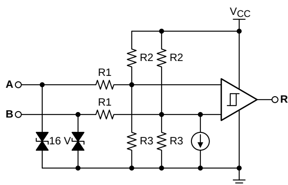
Figure 28. Receiver Inputs
