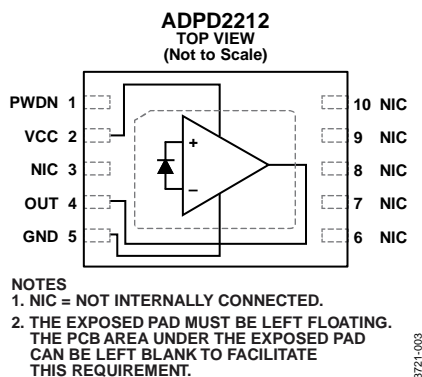
Figure 3. Pin Configuration
