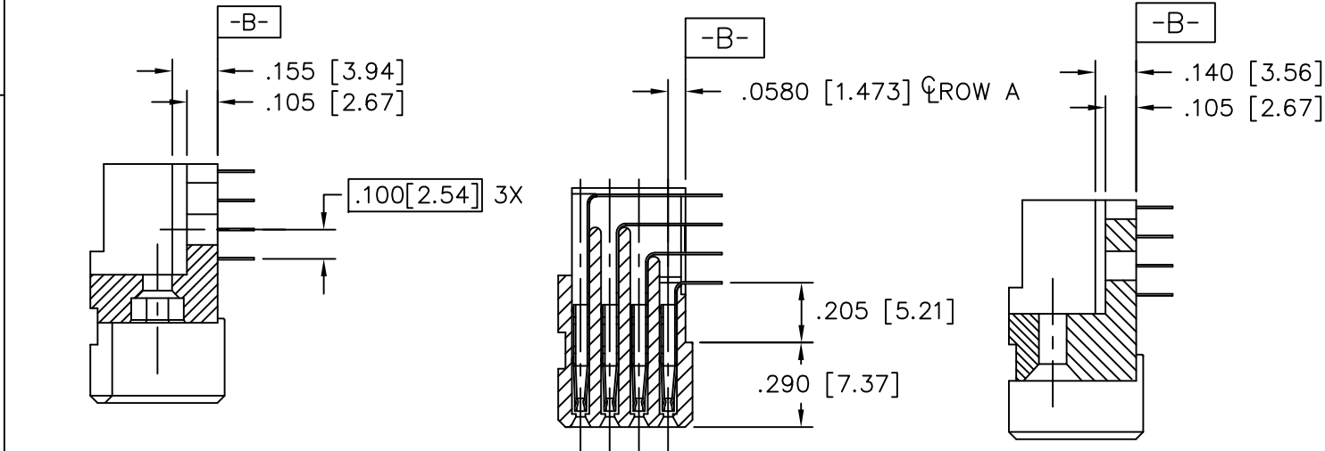
SECTION U—U NO SPECIAL FEATURE
