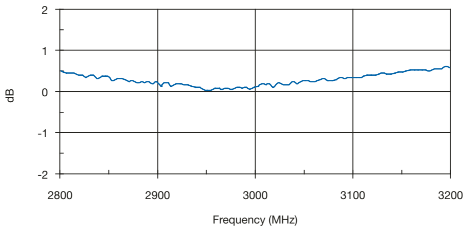
Amplitude Balance
