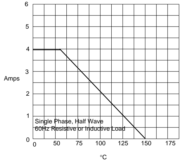
Average Forward Rectified Current - Amperes versus Ambient Temperature - ^{\circ}C
