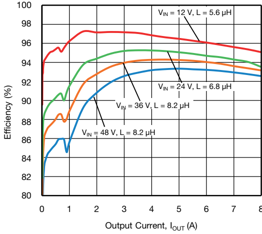
Fig. 17 - SiC472 Efficiency vs. Output Current, VOUT = 5 V
