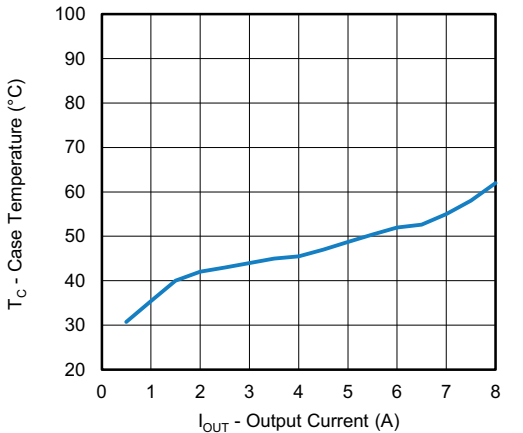
Fig. 19 - SiC472 Load Current vs. Case Temperature, VIN = 48 V, VOUT = 5 V
