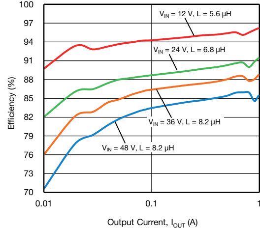
Fig. 20 - SiC472 Efficiency vs. Output Current - Light Load, VOUT = 5 V
