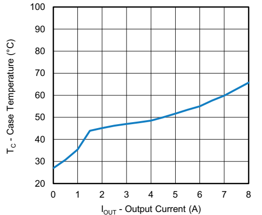
Fig. 22 - SiC472 Load Current vs. Case Temperature, VIN = 48 V, VOUT = 12 V
