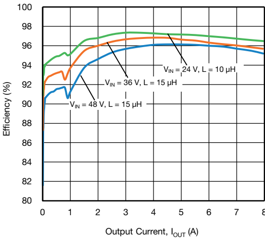
Fig. 18 - SiC472 Efficiency vs. Output Current, VOUT = 12 V
