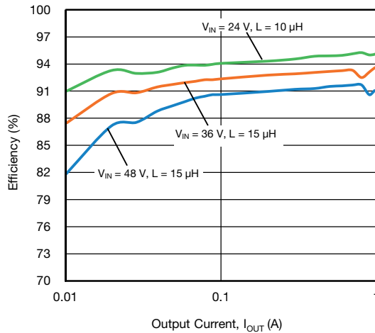
Fig. 21 - SiC472 Efficiency vs. Output Current - Light Load, VOUT = 12 V
