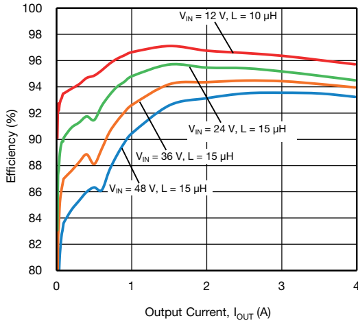
Fig. 29 - SiC474 Efficiency vs. Output Current, VOUT = 5 V
