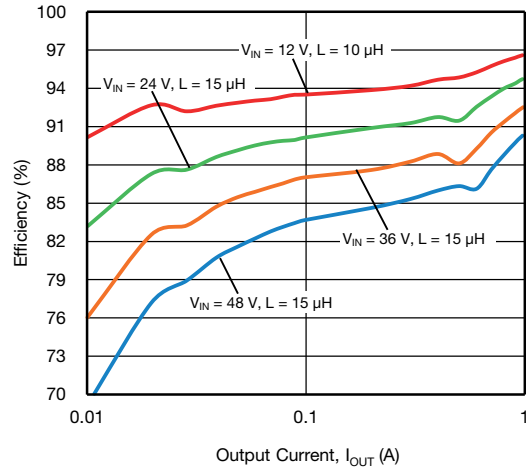
Fig. 32 - SiC474 Efficiency vs. Output Current - Light Load, VOUT = 5 V
