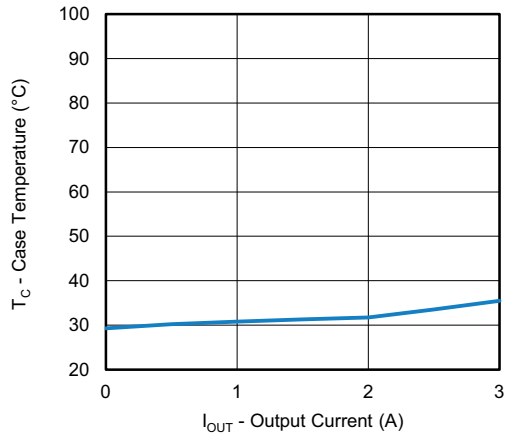
Fig. 31 - SiC474 Load Current vs. Case Temperature, VIN = 48 V, VOUT = 5 V
