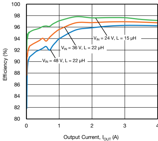
Fig. 30 - SiC474 Efficiency vs. Output Current, VOUT = 12 V
