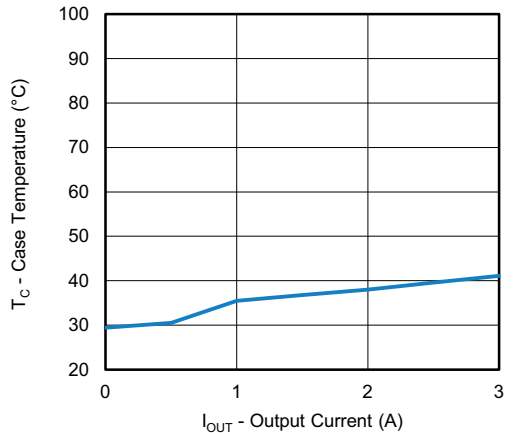
Fig. 34 - SiC474 Load Current vs. Case Temperature, VIN = 48 V, VOUT = 12 V
