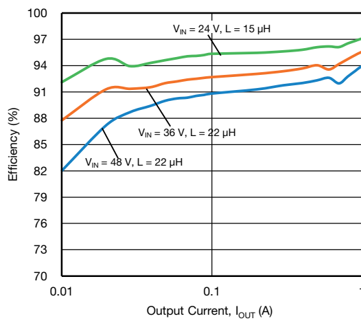
Fig. 33 - SiC474 Efficiency vs. Output Current - Light Load, VOUT = 12 V
