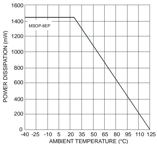
Figure 5. Derating Curve
