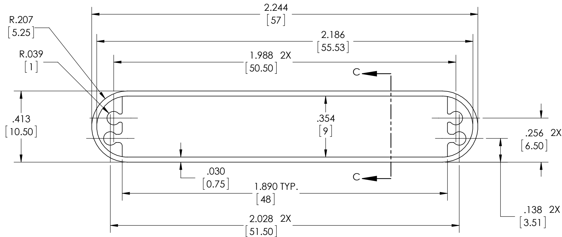
EXTRUSION PROFILE
