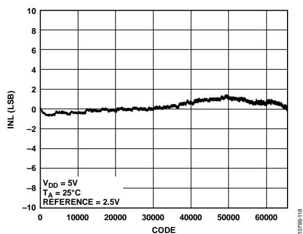
Figure 5. AD5696 INL
