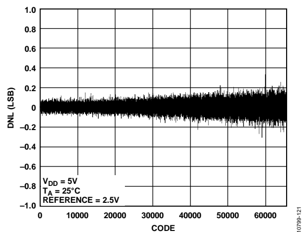
Figure 7. AD5696 DNL
