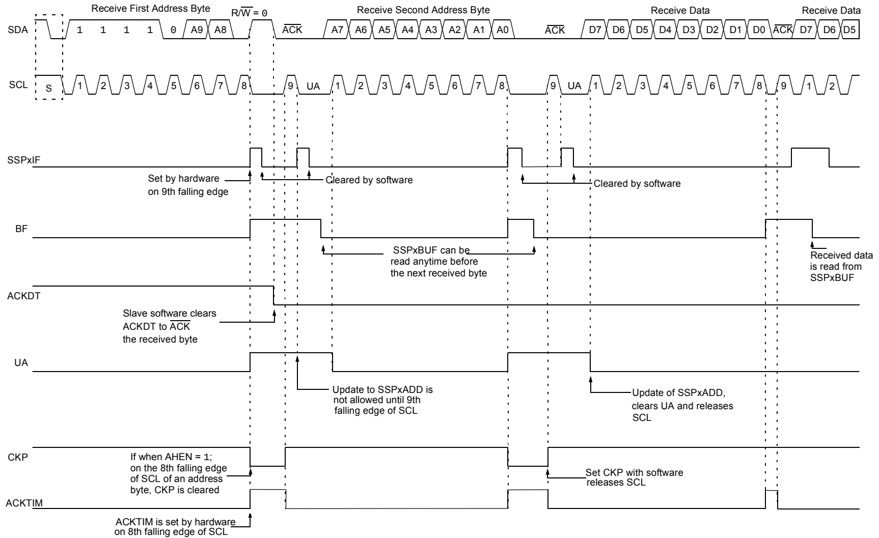
FIGURE 33-21: I 2 C SLAVE, 10-BIT ADDRESS, RECEPTION (SEN = 0, AHEN = 1, DHEN = 0)
