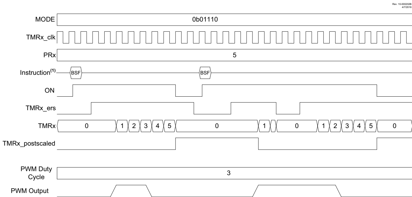
FIGURE 27-11: LOW LEVEL RESET, EDGE-TRIGGERED HARDWARE LIMIT ONE-SHOT MODE TIMING DIAGRAM (MODE = 01110)
