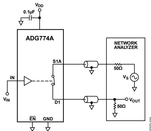
Figure 19. Bandwidth
