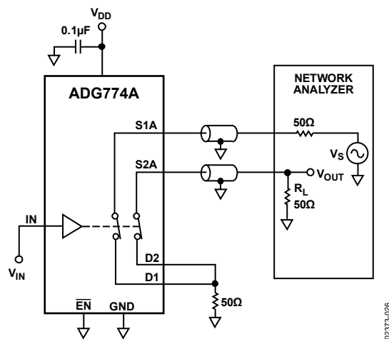
Figure 21. Channel-to-Channel Crosstalk
